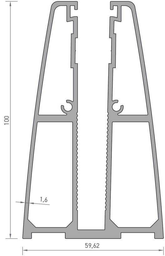
8797 KASA PROFİLİ 2,825 kg/mt
