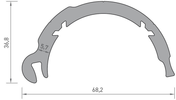
4816 ASKILIK PROFİLİ 1,475 kg/mt
