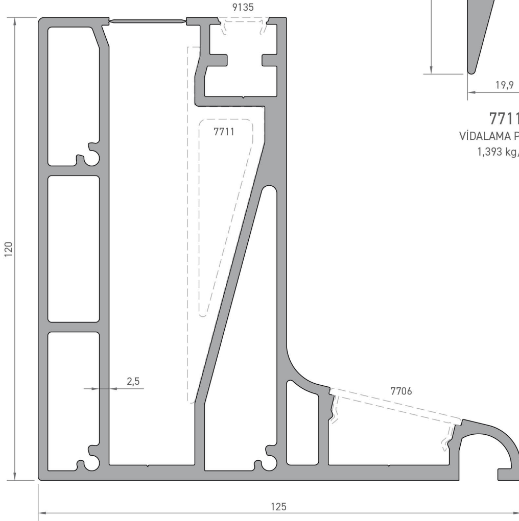
9218 KASA PROFİLİ 5,431 kg/mt
