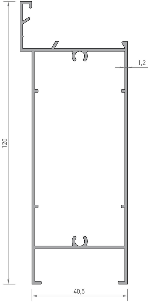
2430 Etek Profili 1,125 kg/mt
