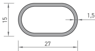
2436 OVAL PANJUR BORU PROFİLİ 0,265 kg/mt
