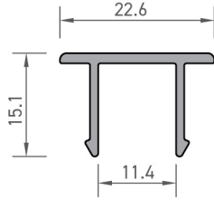
Kapak Profili Cover Profile
