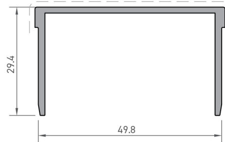
Drenaj Kapak Profili Drainage Cover Profile
