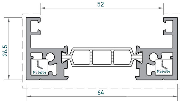
Kanat Profili Sash Profile
