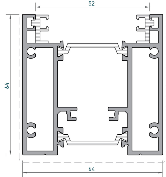
Kanat Profili Sash Profile
