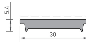
Kanat Kapak Profili Sash Cover Profile
