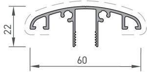
Griyaj Yan Kapak Profili Mullion Cover Profile
