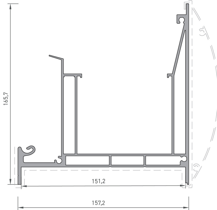
Dere Profili / Gutter Profile
