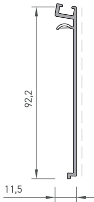
Arka Kapak Profili Middle Cover Profile
