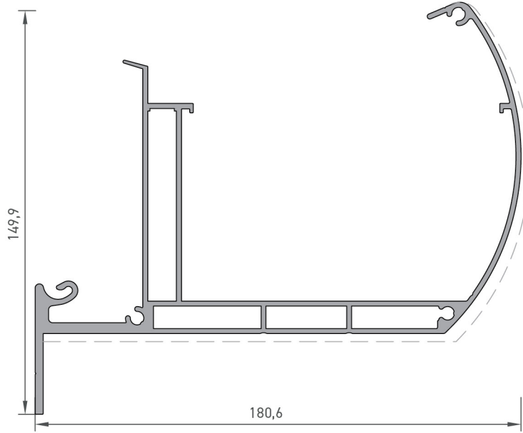
Dere Profili / Gutter Profile
