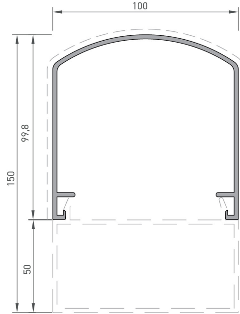
Dikme Kapak Profili / Column Cover Profile
