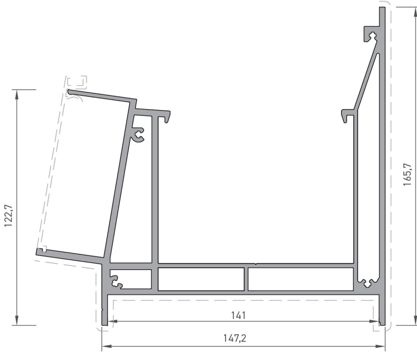
Dere Profili / Gutter Profile
