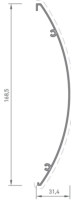
Dere Kapak Profili Gutter Cover Profile
