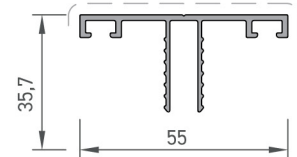
Griyaj Kapak Profili Mullion Cover Profile
