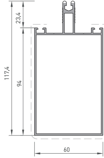
Griyaj Profili / Mullion Profile
