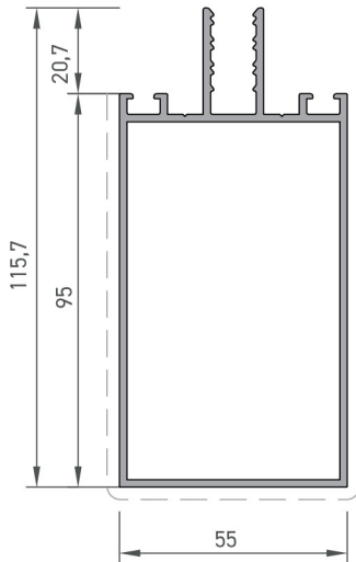
Griyaj Profili / Mullion Profile
