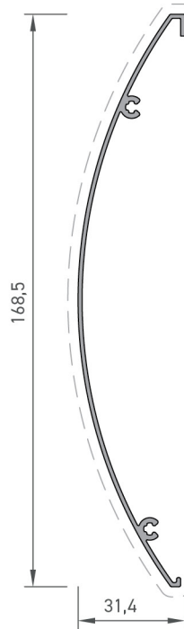
Dere Kapak Profili Gutter Cover Profile
