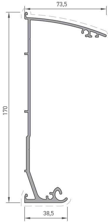
Duvar Sabitleme Profili Wall Fixing Profile
