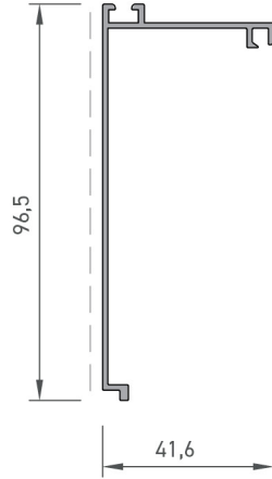
Arka Kapak Profili Middle Cover Profile
