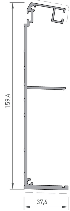
Duvar Sabitleme Profili / Wall Fixing Profile
