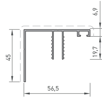
Griyaj Yan Kapak Profili Mullion Side Cover Profile
