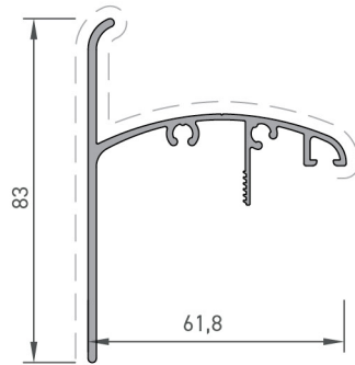
Grijaj Yan Kapak Profili Mullion Side Cover Profile
