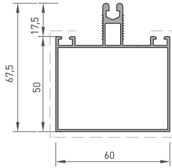
Yatay Griyaj Profili / Transform Profile
