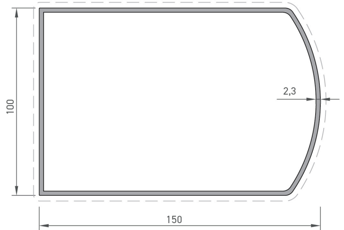
Dikme Kapak Profili / Column Cover Profile
